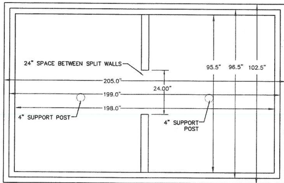
TOP VIEW OF TANK
