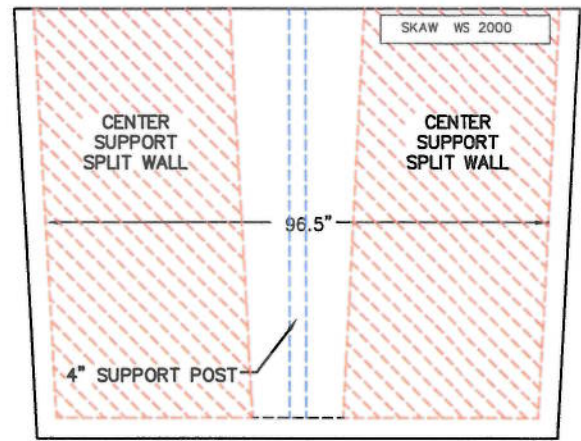
OUTLET END VIEW OF TANK
