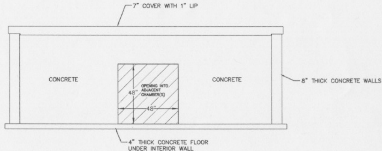
CROSS SECTION OF BLOCK OUT DETAIL (INTERIOR SIDE OR END WALLS)
