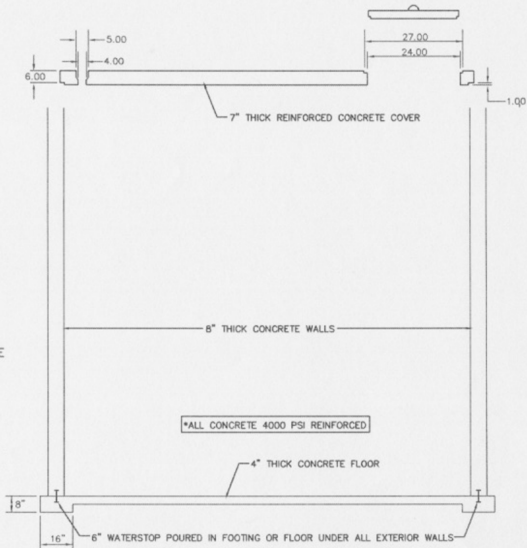
CROSS SECTION OF EXTERIOR FOOTING/WALL
