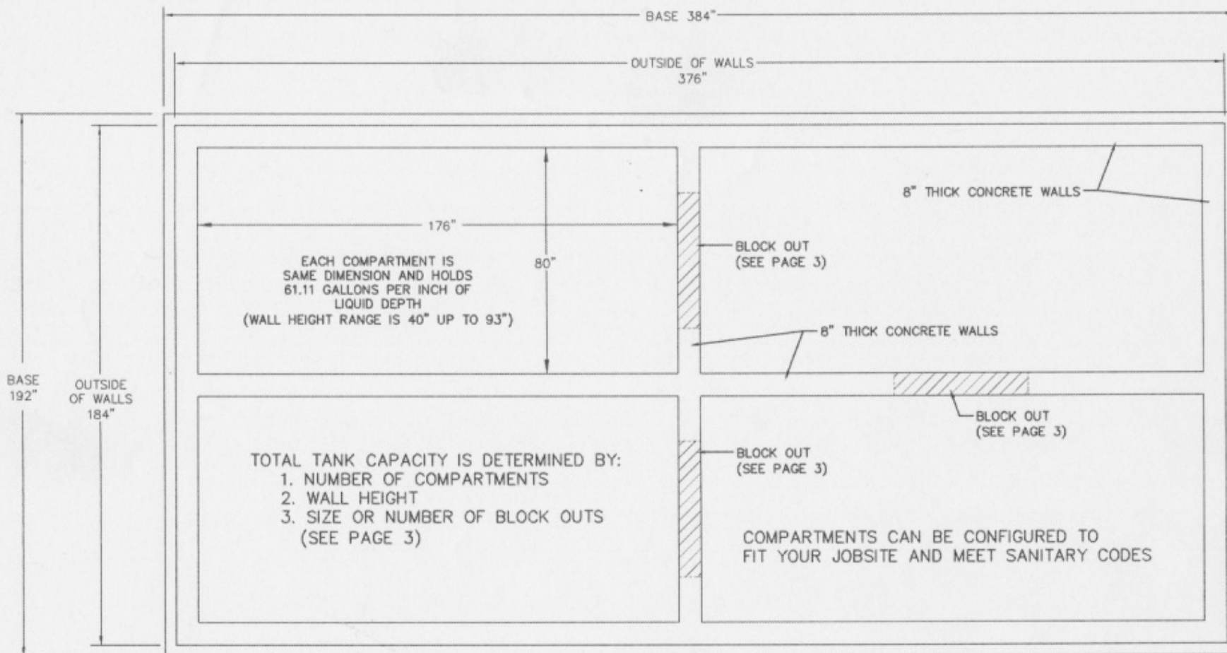
TOP VIEW OF 4 COMPARTMENT TANK (SIDE BY SIDE AND END TO END PLACEMENT)
