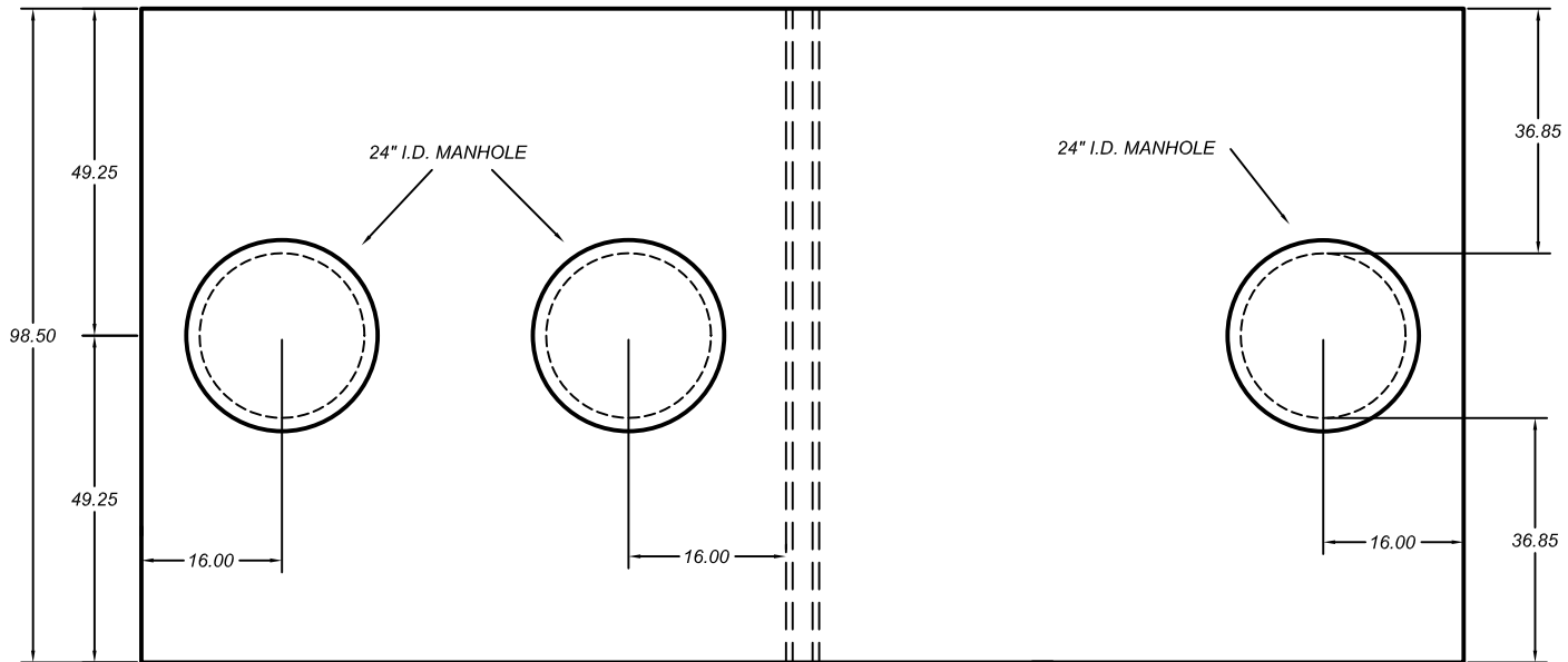
TOP VIEW OF COVER
