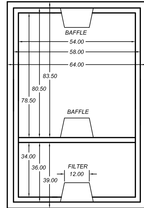
TOP VIEW OF TANK (TAPERED)
