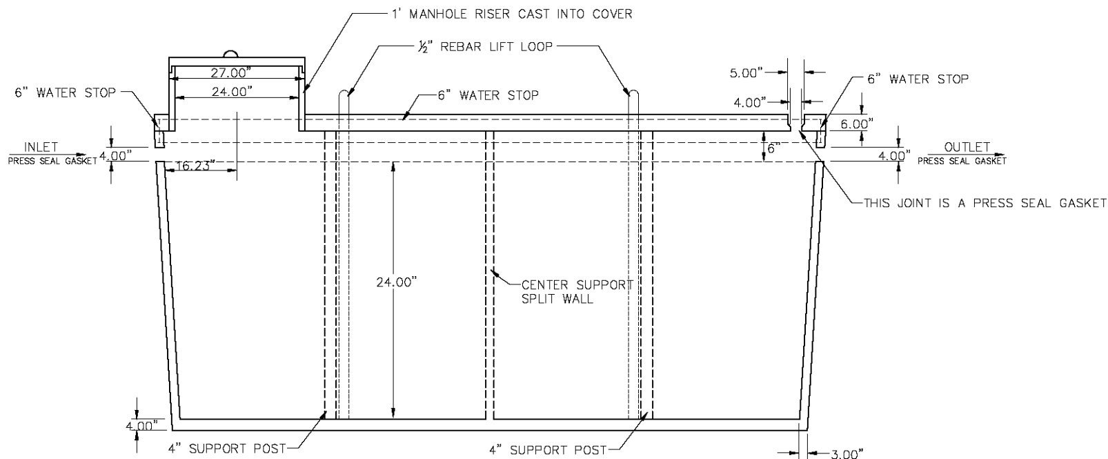
SECTION VIEW OF TANK
